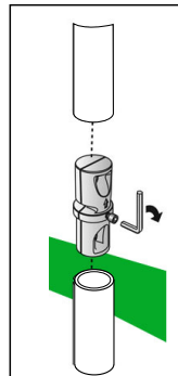
Breakaway Coupler Installation Diagram
