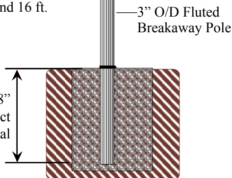
Breakaway Coupler Installation Diagram
