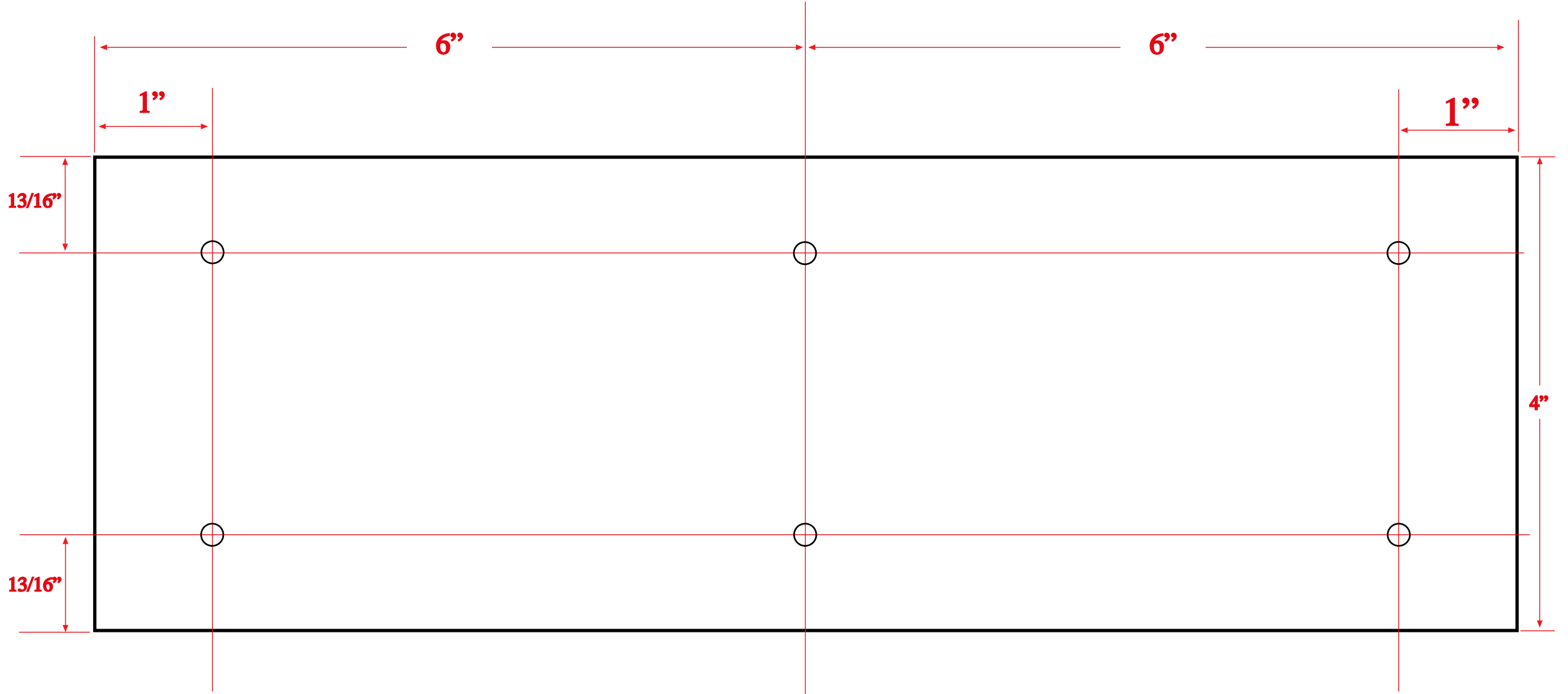
MP-454 Mounting Template
